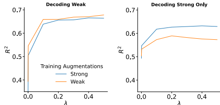
Figure 7: Augmentation parameter decoding performance on held-out test images for networks trained using either strong or weak transformations. In the left panel we plot the decoding performance for weak transformations only, and in the right panel the performance for strong transformations only (which are not seen by the weak-trained networks during pretraining).
