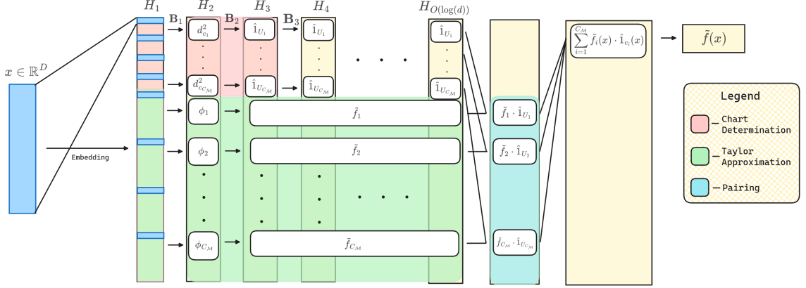
Figure 1: Diagram of the transformer architecture constructed in Theorem 2. T computes approximations of f(x) on each local chart U_n \subseteq \mathcal{M} by first projecting x to the tangent coordinates in \mathbb{R}^d via \phi_n(x) and then approximating f(x) with local Taylor polynomials. A shallow sub-network computes indicators \mathbf{1}_{U_n} for each local chart in parallel. The results of the two sub-networks are then multiplied together and summed to produce the final result. Here H_i denotes the embedding matrix before the i th transformer block B_i .
