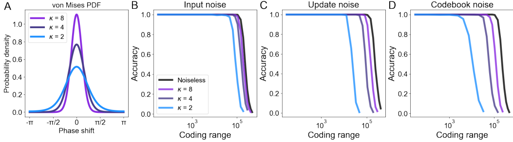
Figure 3: Recovery of encoded positions is robust to multiple kinds of noise. A) Visualization of the von Mises weight distribution. Note that the magnitude of the noise is inversely proportional to \kappa , and that the variance of the phase perturbation is much larger than the distance between the discrete states of phasors. B-D) Visualizations of accuracy as a function of coding range and \kappa for three separate cases: input noise (B), update noise (C), and codebook noise (D). Cases are shown in order of increasing difficulty. The resonator network maintains perfect accuracy up to a point, after which accuracy decays at an earlier point than the noiseless dynamics (black curve).
