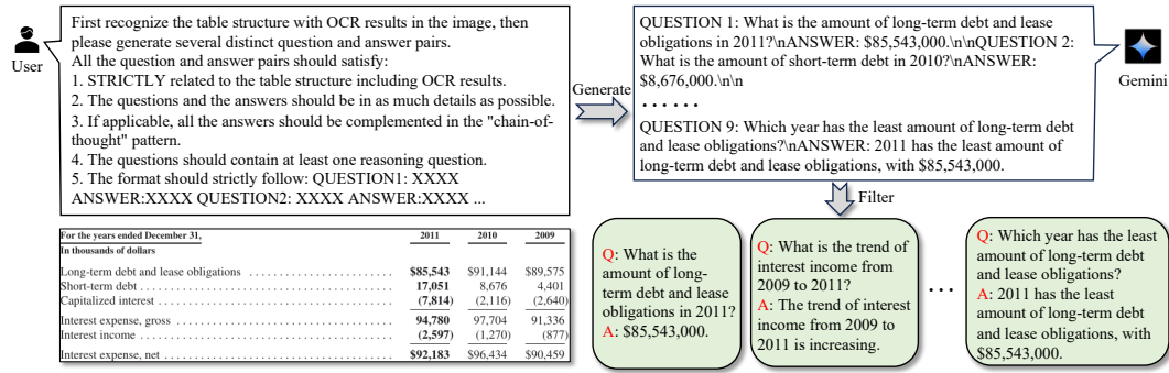
Figure A1: The illustration of an example for generating QA pairs with the powerful LVM, Gemini Pro [93]. The prompt includes several key rules to ensure the response quality as much as possible.
