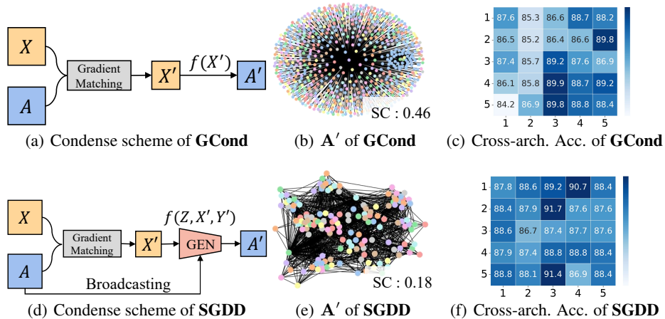
Figure 1: (a) and (d) illustrate that the pipelines of SGDD and GCond [37]. One can find that SGDD broadcast A from the original graph to the generation of A' while GCond synthesizes A' via the operation f(\cdot) (e.g., pair-wise feature similarity [74]) on X' . We also show the condensed graph and its shift coefficient (SC) of GCond and SGDD in (b) and (e), respectively. Note that we introduce SC as an approximation of the LED shift. We show the cross-architecture performance of GCond and SGDD in (c) and (f), 1, 2, 3, 4, and 5 denote APPNP [42], Cheby [13], GCN [41], SAGE [26], and SGC [92], more cross-architecture results can be found in Tab. 2.
