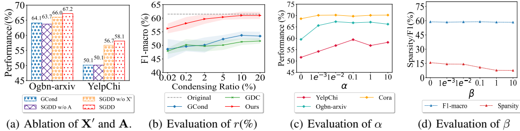
Figure 4: (a) Ablation of components in SGDD. (b) Evaluation of the scalability of SGDD. (c) and (d): the trade-off parameters analysis on \alpha and \beta .
