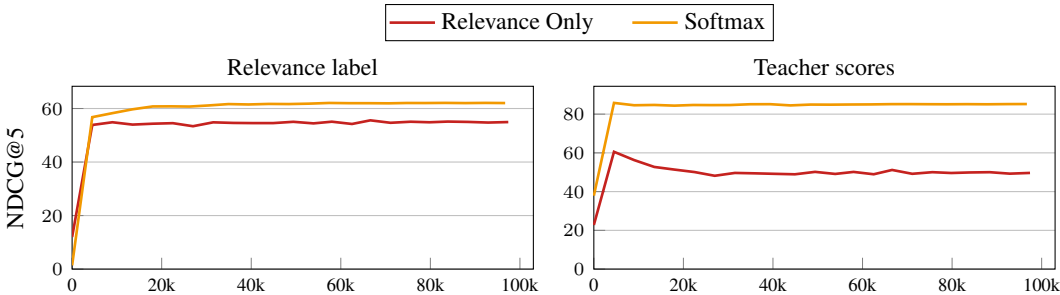
Figure 1: The performance of Relevance Only and Softmax on relevance label and teacher scores for the NQ ranking distillation task. NDCG is used since teacher scores are real-valued.
