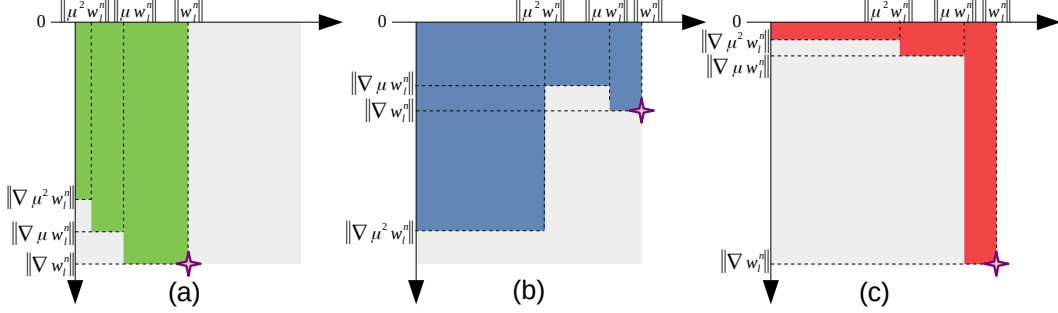
Figure 1: Illustration of possible limitations of traditional pruning criteria for 3 distinct cases and neurons (a,b,c). For a neuron n at layer l we plot the weights norm \|\mu^s w_i^n\| and corresponding gradients norm \|\nabla \mu^s w_i^n\| of different neurons (a, b and c) for different powers of \mu^s \in ]0; 1[ corresponding to a path towards zeroing out this neuron. Magnitude-based approaches (a) remove low magnitude neurons regardless of the sensitivity (gradient norm) of the predictive function w.r.t. these neurons. Gradient-based approaches (b) are limited by the intrinsic locality of the gradient, and abruptly setting a neuron weights to zero may break this locality principle. Conversely, our integrated gradient-based approach (c) will prune neuron although it initially has a high magnitude and gradient, integrating its gradient variations along a path down to zero magnitude.
