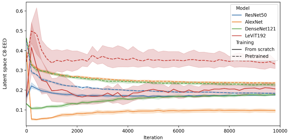
Figure 4: The latent space C_8 -EED measured every 200 training iterations (for a total of 10,000 iterations) for a range of model architectures that were initialized with either random or ImageNet pretrained weights. Confidence intervals are over 5 randomly initialized models for ‘from scratch’ and 5 independent trainings for ‘pretrained’.
