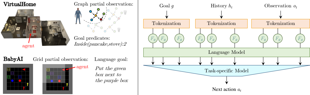
Figure 1: Environments (left) : Different environments have different types of observations and goals. Our approach (right) : We use pre-trained LMs as a general framework for interactive decision-making by converting policy inputs into sequential data. Such a method enables effective combinatorial generalization to novel tasks.
