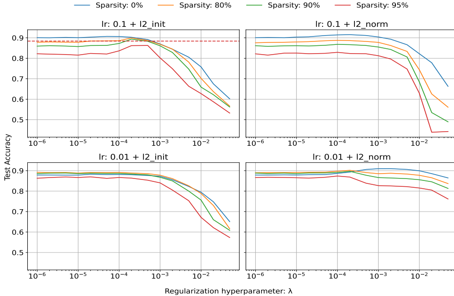
Figure 3: Test accuracy of ResNet20 trained on CIFAR10 when regularization term is added. Top row shows the results of the large learning rate (0.1) and bottom row shows those of the small learning rate (0.01). Left: l2\_init , Right: l2\_norm . The dashed red line in the top left shows the unpruned baseline with the small learning rate (0.01).
