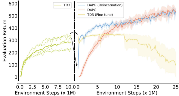
Figure 5: Reincarnating RL on humanoid:run. (Panel 1) . We observe that TD3 nearly saturates in performance after training for 10M environment steps. The dashed traces show individual runs while the solid line shows the mean return. (Panel 2) . Reincarnated D4PG performs better than its tabula rasa counterpart until the first 10M environment steps and then converges to similar performance (with lower variance). Furthermore, training TD3 for a large number of steps eventually results in performance collapse. We use identically parameterized MLP critic and policy networks with 2 hidden layers of size (256, 256) for TD3 but larger networks with 3 hidden layers for D4PG. Shaded regions show 95% CIs based on 10 seeds.
