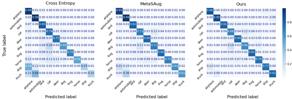
Figure 2: Confusion matrices of the cross-entropy training, MetaSAug and ours on CIFAR-LT-10 with the imbalance factor 200. We rank classes by the frequency, i.e. , frequent (left) and rare (right).
