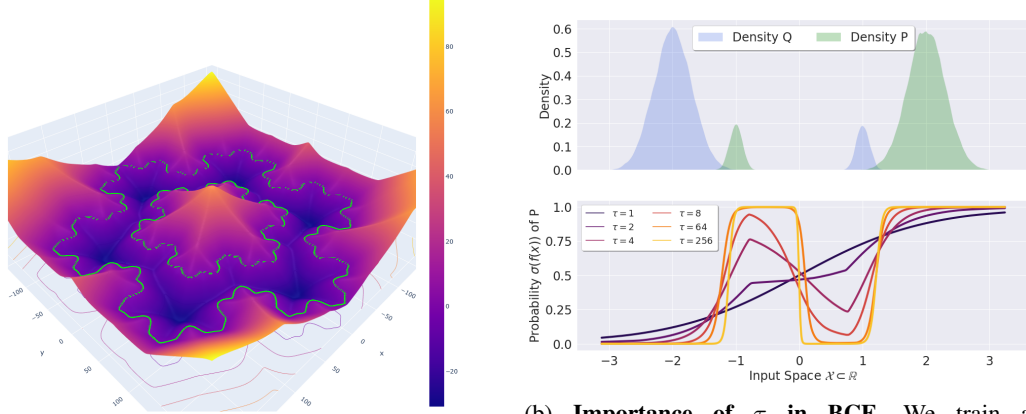
(b) Importance of \tau in BCE. We train a LipNet1 network with BCE and different values for \tau . We chose a toy example where P and Q are Gaussian mixtures with two modes of weights 0.9 and 0.1. We highlight the different shapes of the minimizer \sigma \circ f as function of \tau . High values of \tau leads to better fitting, whereas for lower \tau the small weights Gaussian of the mixture are treated as noise and ignored.
