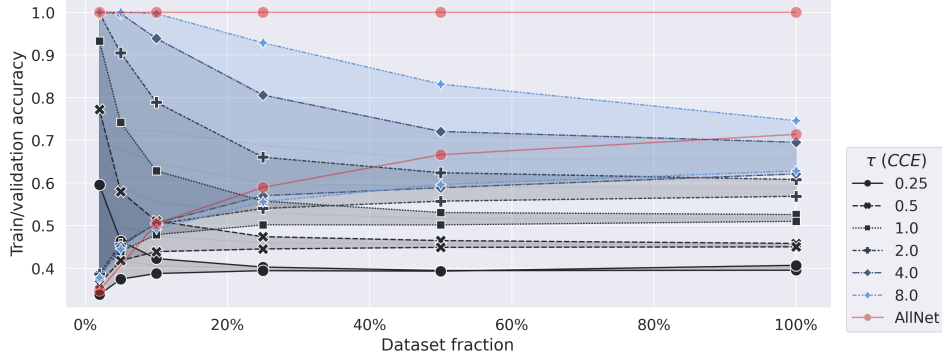
Figure 4: Link between LipNet1 and generalization gap, dataset size and cross-entropy temperature. We train a CNN on different fractions of the CIFAR10 train set (2%, 5%, 10%, 25%, 50% and 100% on x -axis) with different values of temperature \tau (highlighted by different colors). Train (resp. validation) accuracy forms the upper (resp. lower) bound of each envelope. As \tau increases, more samples are required to reduce the generalization gap. Conversely, training a LipNet1 network with small \tau is equivalent to training a Lipschitz network with small L : the network generalizes well but the accuracy reaches a plateau (under-fitting). The AllNet network (in red) severely overfit: the generalization gap is large and validation accuracy corresponds to the limit that would reach a LipNet1 as \tau increases. See appendix J for detailed experimental setting.
