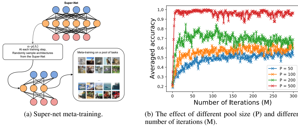
Figure 3: Figure 3a is an overview of the super-net meta-training. Figure 3b shows how different parameters in the Adaption strategy can affect accuracy.
