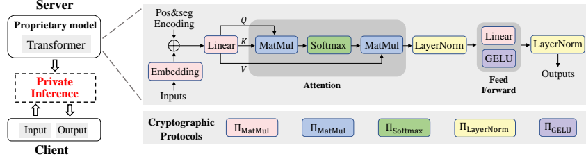
Figure 1: Overview of private Transformer inference
