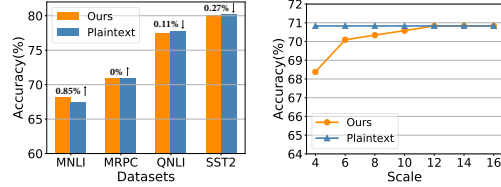
Figure 6: Accuracy comparison with plaintext
