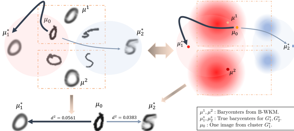
Figure 3: Visualization of misclassification for the barycenter-based Wasserstein K -means (B-WKM) on a randomly sampled subset from MNIST (200 digit "0" and 100 digit "5"). The plot at the bottom is an example of misclassified image. The right plot is the abstraction of the images in the Wasserstein space. The color depth indicates the frequency of the distributions. Red and blue colors stand for distributions belong to true clusters "0" and "5".
