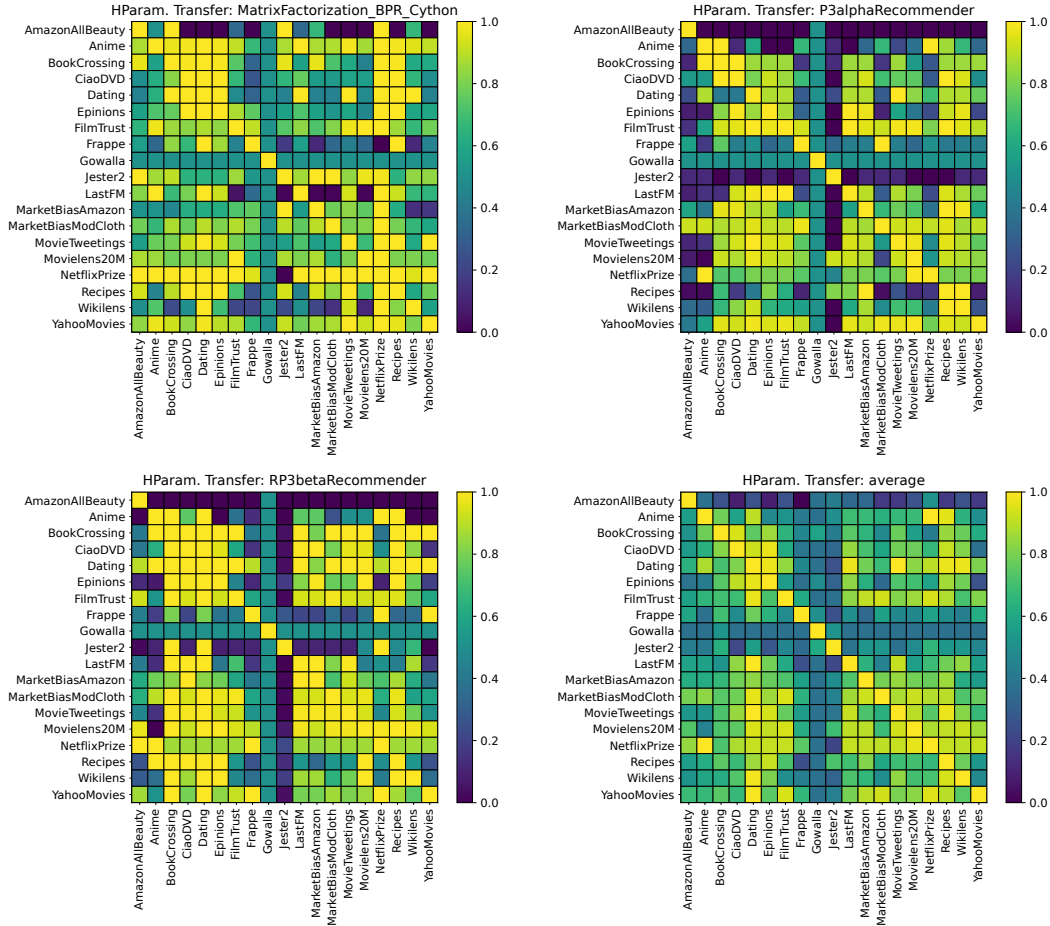
Figure 3: Transferability of hyperparameters across datasets, for three different algorithms, and the average of all algorithms (bottom right). For each plot, row i , column j denotes the relative performance of an algorithm tuned on dataset i and then evaluated on dataset j . A value close to 1 indicates that the hyperparameters transfer well from i to j , while a value close to 0 indicates that the hyperparameters transfer poorly.
