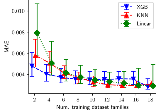
Figure 4: Three basic meta-learners (KNN, linear regression, and XGB) are trained randomly-selected dataset families to predict performance metric \text{PREC}@10 . As more dataset families are added, the meta-learners are better able to predict rec-sys algorithm performance, suggesting that our dataset meta-features are useful for predicting rec-sys algorithm performance. Vertical axis shows mean absolute error (MAE), over all folds of leave-one-out validation, and 200 random trials; in each trial a different set of training datasets are chosen. Error bars show the 40th and 60th percentile.
