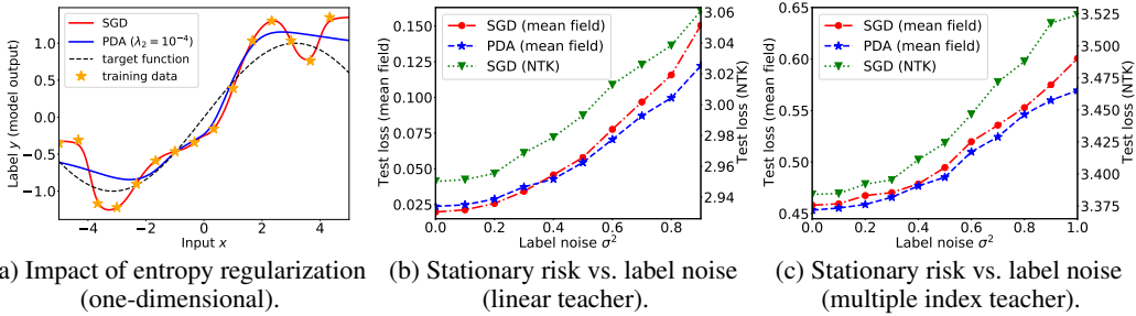
Figure 5: (a) 1D illustration of the impact of entropy regularization in two-layer tanh network: PDA (blue) finds a smoother solution that does not interpolate the training data due to entropy regularization. (b)(c) Test error of two-layer tanh network trained till convergence. PDA (blue) becomes advantageous compared to SGD (red) when labels become noisy, and the NTK model (green, note that the y-axis is on different scale) generalizes considerably worse than the mean field models.
