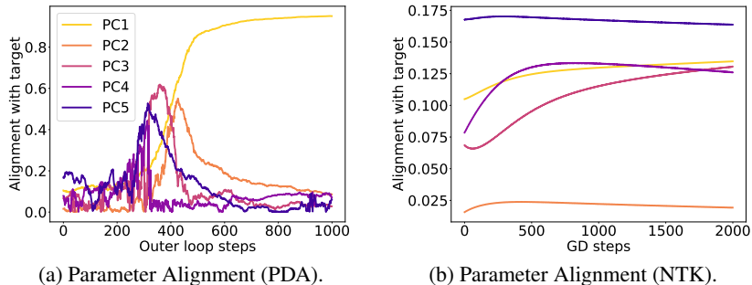
Figure 6: Cosine similarity between the target vector w^* and the top-5 singular vectors (PC1-5) of the weight matrix during training. The learned parameters “align” with the target function under the mean field parameterization (a), but not the NTK parameterization (b).
