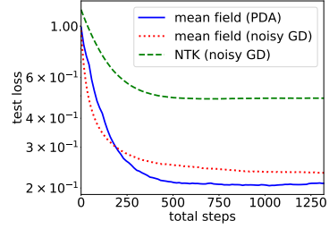
Figure 3: Test error of mean field neural networks ( \alpha = 1 ) trained with noisy GD (red) and PDA (blue), and network in the kernel regime ( \alpha = 1/2 ) optimized by GD (green).
