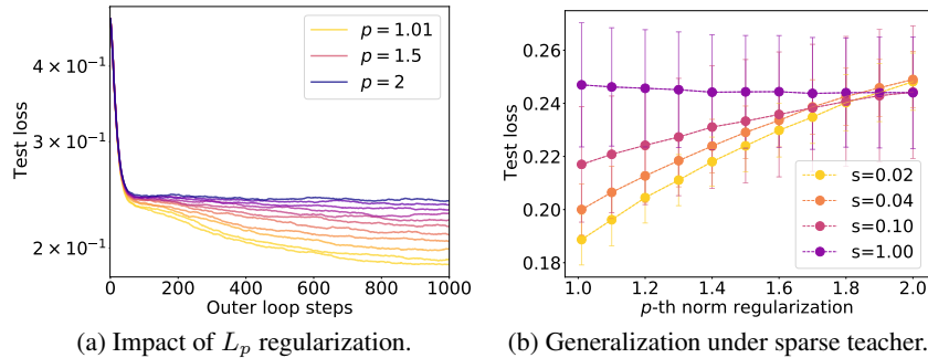
Figure 4: PDA with general \ell_p regularizer (objective (36)). (a) Generalization error vs. training time in learning a 1-sparse target function. (b) generalization error vs. sparsity of the target function s .
