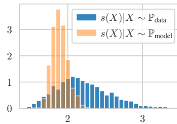
Figure 3: Sampling distribution for the OoD test (blue) and the GoF test (orange). While the same statistic s(X) is used in both cases, the p -values are computed differently depending on which test we perform.
