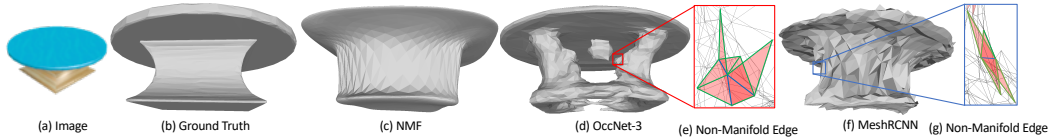
Figure 10: Implicit methods: OccNet fails to give meshes that are singly connected and MeshRCNN has poor normal consistency along with severe self-intersections. Both OccNet and NMF has non-manifold edges (shown as zoomed out insets). NMF generates meshes that are visually appealing with higher manifoldness.
