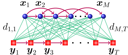
Figure 1: We propose a framework, based on a generalization of the facility location problem, for the summarization of sequential data. Given a source set of items \{x_1, \dots, x_M\} with a dynamic transition model and a target set of sequential items (y_1, \dots, y_T) , we propose a framework to find a sequence of representatives from the source set that has a high global transition probability and well encodes the target set.
