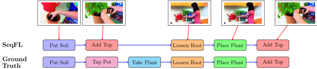
Figure 6: Ground-truth and the summarization result of our method (SeqFL) for the task ‘Repot a Plant’.
