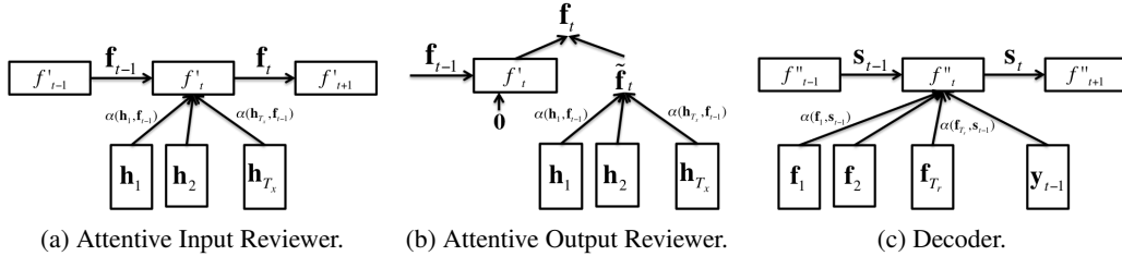
Figure 2: Illustrations of modules in the review network. f' and f'' denote LSTM units.
