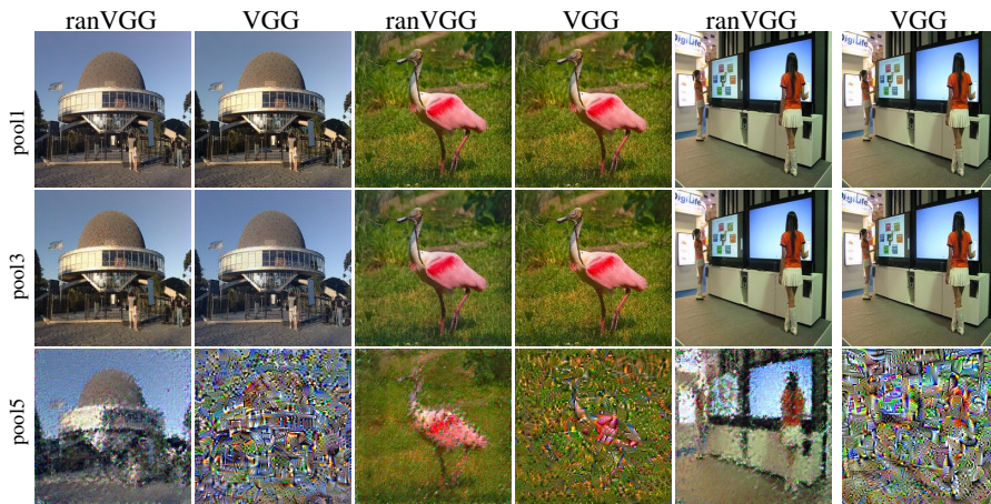
Figure 2: Reconstructions from different pooling layers of the untrained ranVGG and the pretrained VGG. ranVGG demonstrates a higher perceptive quality, especially on the higher layers. The pretrained VGG could rarely reconstruct even the contours from representations of the fifth pooling layer.
