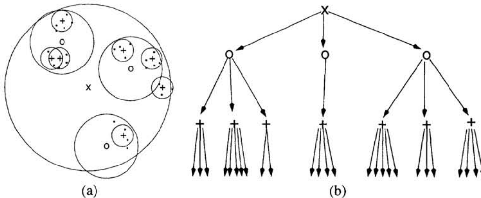
Figure 1: The basic idea of the hierarchical mixture model. (a) \times denotes the root of the tree, the second level centres are denoted by o 's and the third level centres by + 's. Data is generated from the third level centres by sampling random points from Gaussians whose means are the third level centres. (b) The corresponding tree structure.
