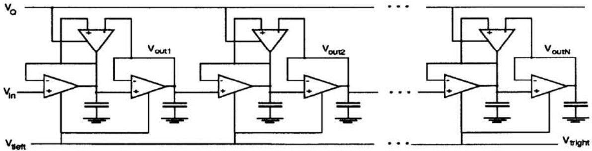
Figure 2: Cochlea circuit
